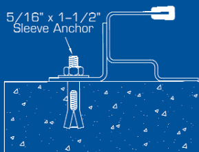
Masonry Mount
