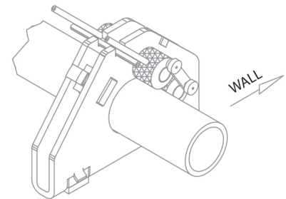
TENSIONER ASSEMBLY - 1-5/16" ONE EACH PER DOOR
