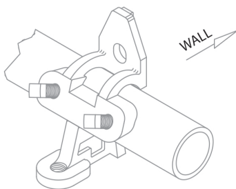
CAST AXLE SUPPORT BRACKET - 1-5/16" HAND CHAIN OPERATION ONE EACH PER DOOR
