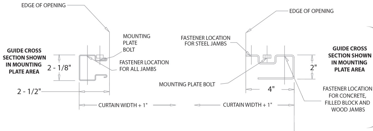
FIGURE 3 GUIDE INSTALLATION
