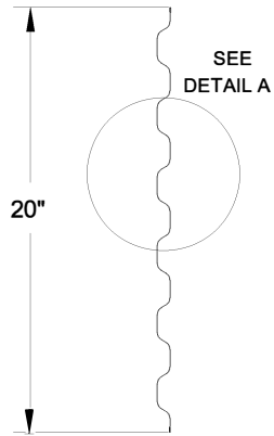
26 GA CURTAIN PANEL DETAIL
