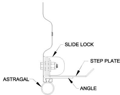
BOTTOM BAR ASSEMBLY
