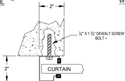
CONCRETE/MASONRY JAMBS
