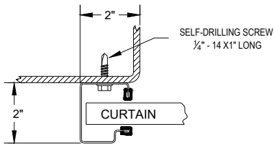
STEEL JAMBS
