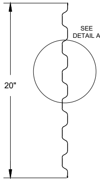
26 GA CURTAIN PANEL DETAIL
