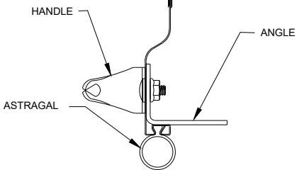
BOTTOM BAR ASSEMBLY
