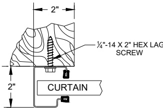
WOOD JAMBS
