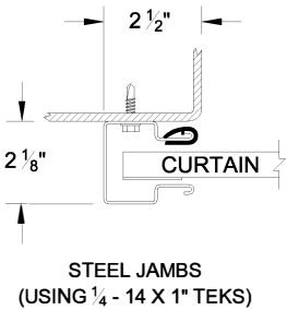
16 GA GUIDE MOUNTING DETAIL
